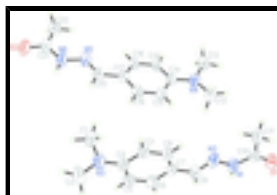
Fig. 1. The asymmetric unit of the title compound. Displacement ellipsoids are drawn at the 40% probability level. Dashed lines indicate hydrogen bonds.
