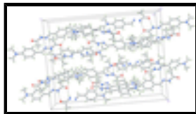
Fig. 2. Crystal packing of the title compound. Hydrogen bonds are shown as dashed lines.
